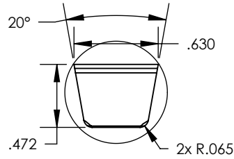
DETAIL B SCALE 1 : 1
